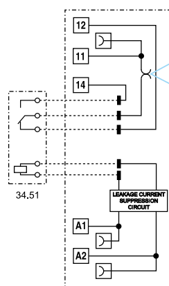
93.63.3 / 93.66.3
