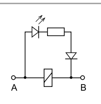
C: Option 3, 5, 54 LED + Freilaufdiode (AC)
