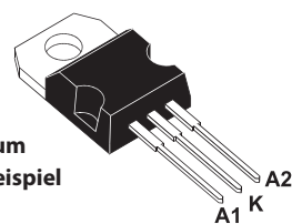
TO-220AB STPS30L40CT
